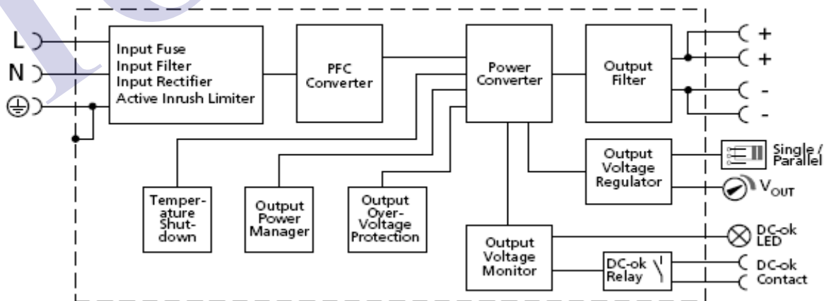
Functional diagram
